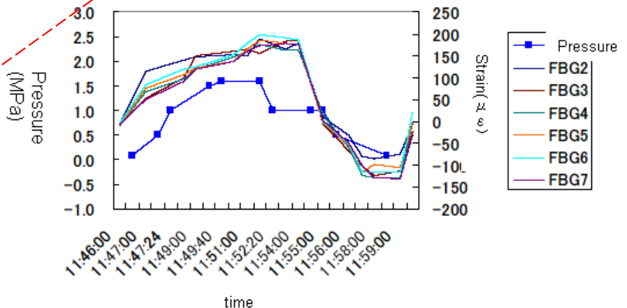
Linear strain movement along with pressure operation
