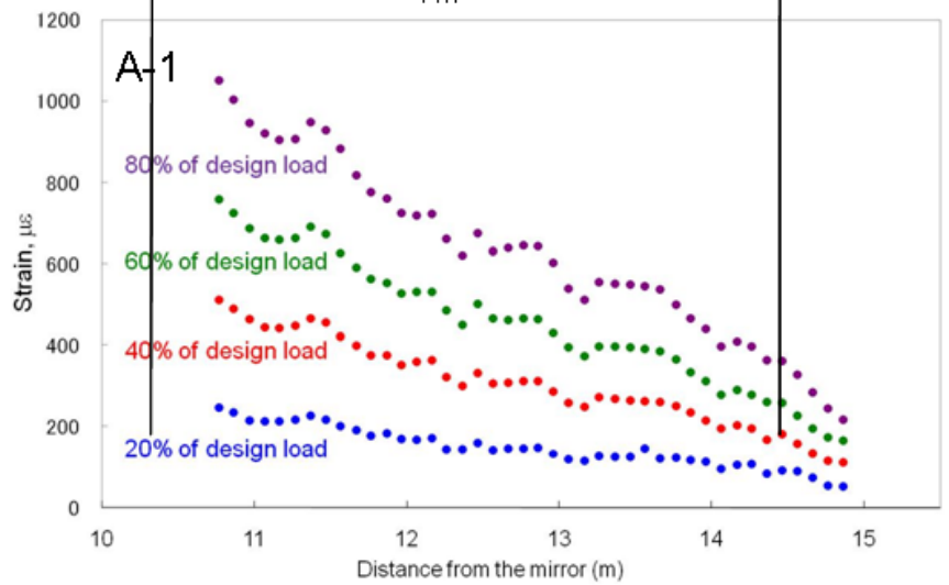
Strain distribution at different loads
